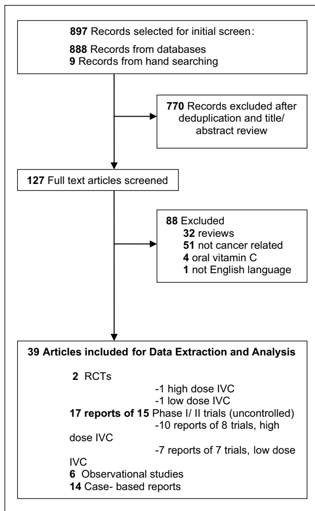
Figure 1. Literature flowchart.
